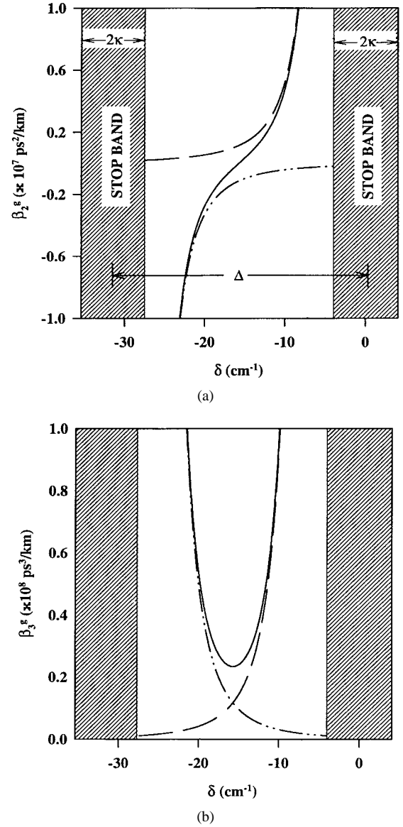
Fig. 1. (a) Group-velocity dispersion and (b) third-order dispersion as functions of \delta for a single grating centered at \delta = 0 (dashed line) and \delta = -\Delta (dot-dashed line), and for two cascaded gratings (solid line). The parameters used are \kappa = 4 \text{ cm}^{-1} , \Delta\nu = 100 \text{ GHz} ( 31.4 \text{ cm}^{-1} ).
