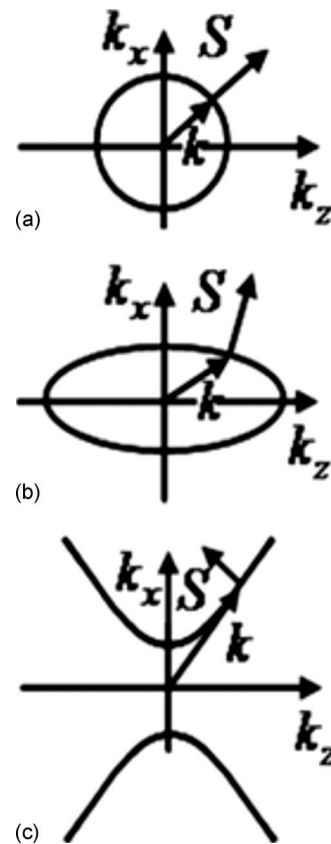
Fig. 3. Isofrequency curves and relative directions of the wave vector k and the Poynting vector S for (a) isotropic material, (b) material with \epsilon_x, \epsilon_z > 0 , (c) material with \epsilon_x < 0, \epsilon_z > 0 [43].
